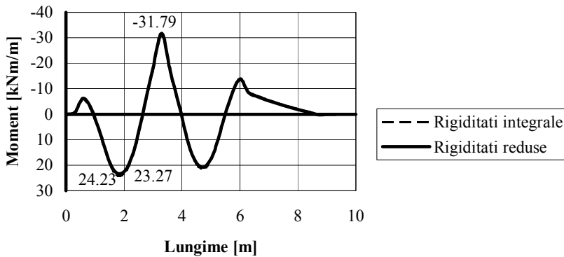
Figure 4 Diagram of bending moments M_x , for x=8.46\text{m}
