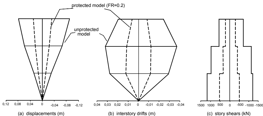
Figure 3.6 Response Envelope for 3-Story Model (FR=0.2)
