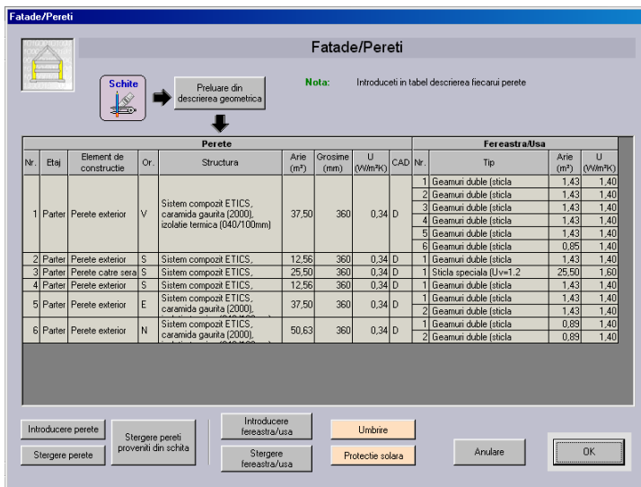
Fig. 7. Detailed definitions of building elements (walls in this case)
