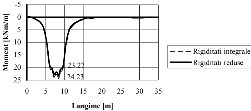
Figure 3 Variation of bending moment M_x in the field of the plate ( y=1.80\text{m} )
