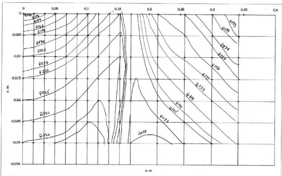
Figure 4. Curves of equal values of OSSR for MASF16 asphalt mixture at 23°C
